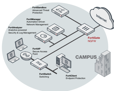
FortiGate 200F Campus Deployment (NGFW)
