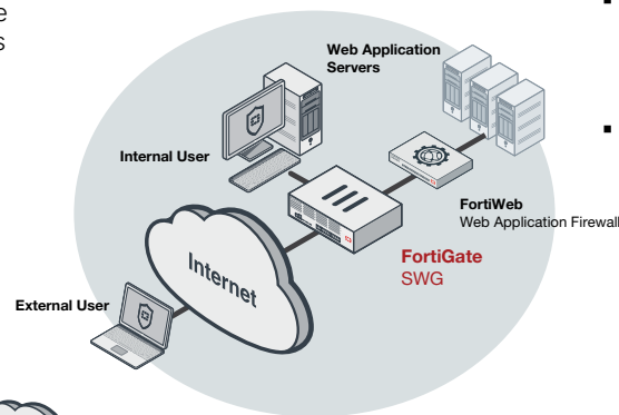
FortiGate 200F SWG Deployment
