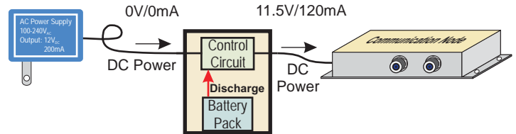
Figure 3 - Configuration with NeverOff on Battery Power
