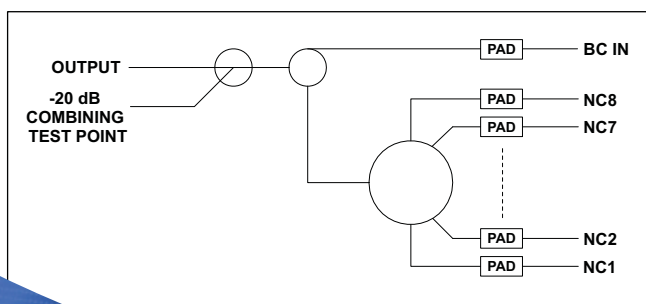
Functional Schematic
